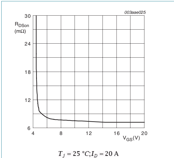
Fig 5. Drain-source on-state resistance as a function of gate-source voltage; typical values.
